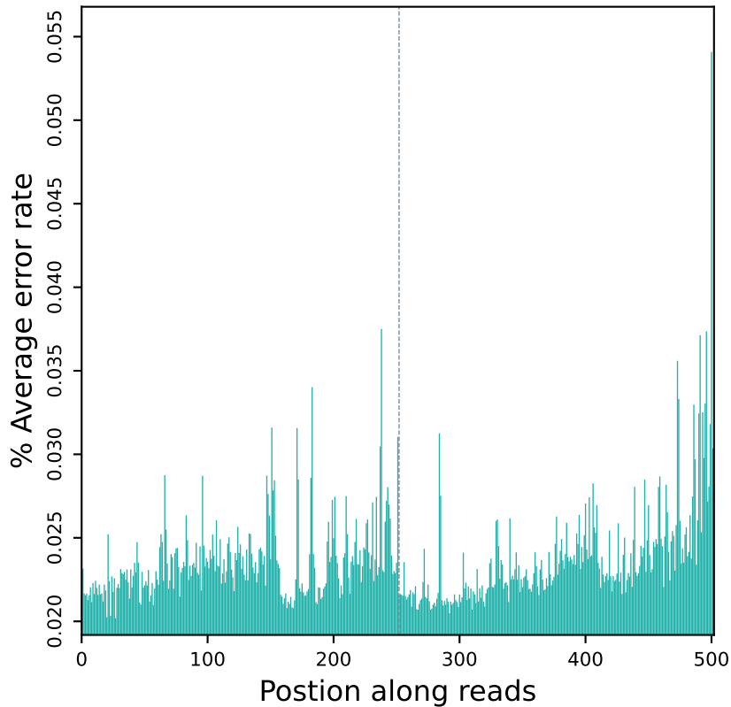
Error rate distribution along reads (CKH1)
